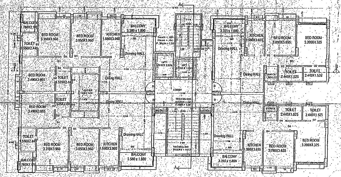
TYPICAL FLOOR PLAN 1st TO 12th FLOOR
